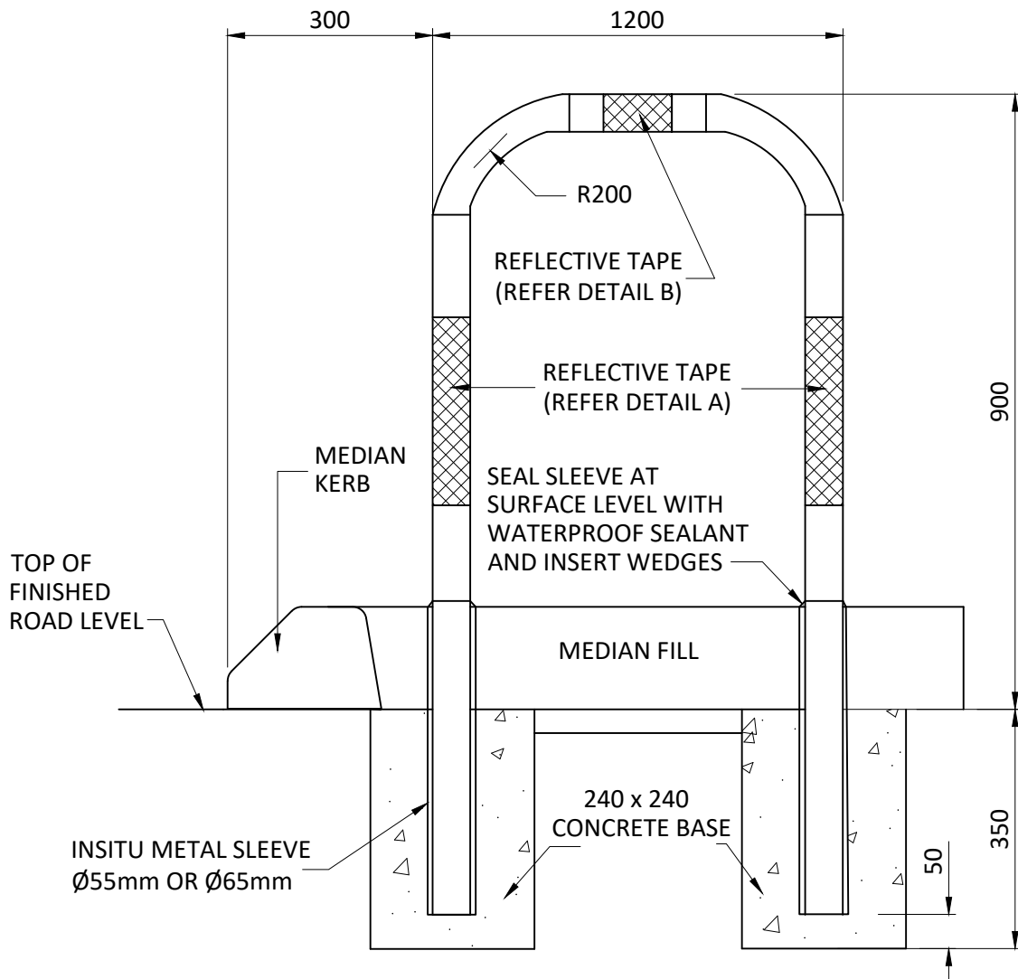
DETAIL B
